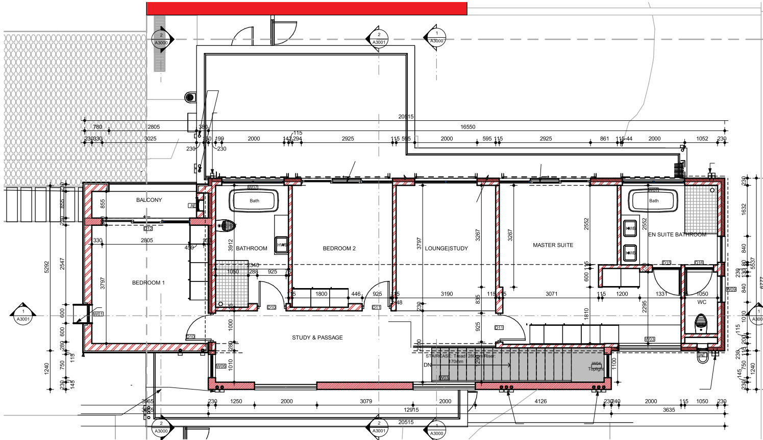
1 | 02_ FIRST FLOOR 1 : 50
